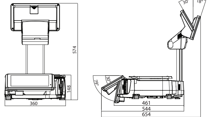
12.1 INCH SELF-SERVICE
