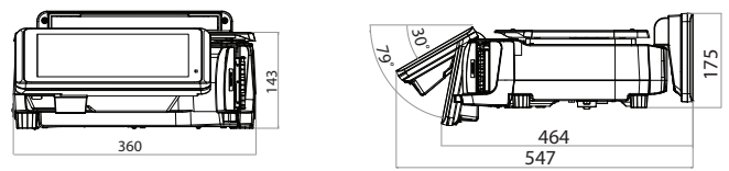
BENCH PLUS
