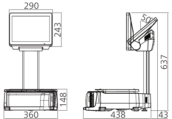
12.1 INCH SELF-SERVICE
