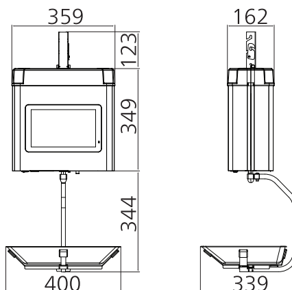
HANGING
