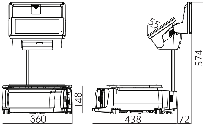
ELEVATED
